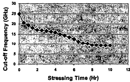
Fig. 3 Cutoff frequency degradation subject to stress
