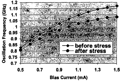
Fig. 8 Tuning range degradation
