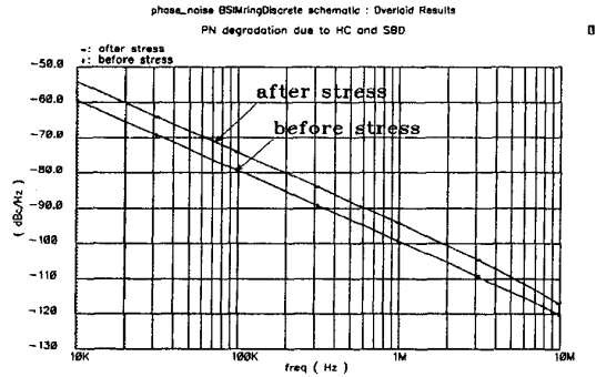
Fig. 7 SpectraRF simulation results
