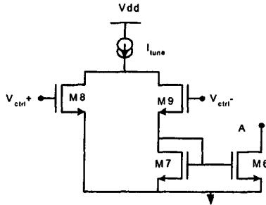
Fig. 5 A control circuit
