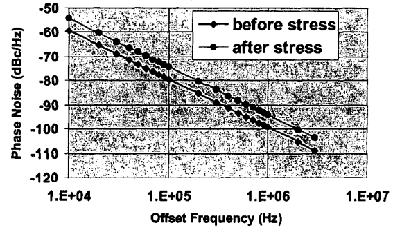
Fig. 6 Predicted phase noise versus offset frequency
